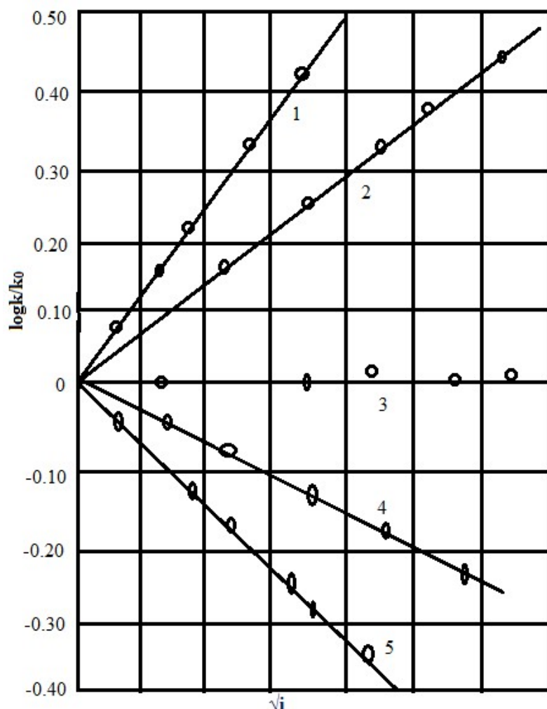
Fig 2: Rate constant variation with ionic strength
